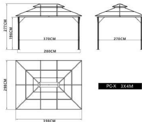
Dimensional Drawing of PC-X
