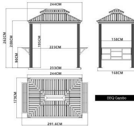
Dimensional Drawing of PC-X
